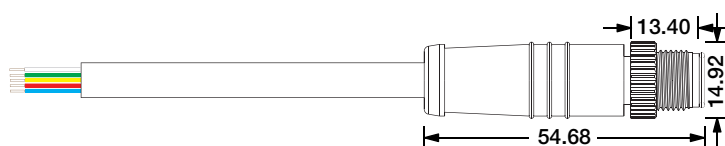
Male Connector M12-M-5C-20AWG-D6-W-0327-S
