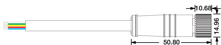
Female Connector M12-F-5C-20AWG-D6-W-0327-S
