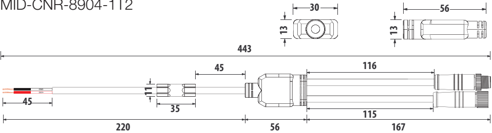
Middle Power Connector (1 to 2) MID-CNR-8904-1T2
