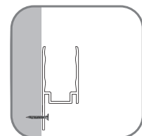
Installation Way
