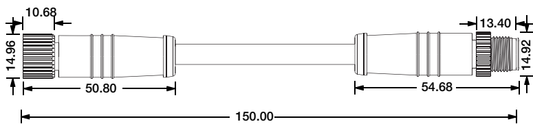
Positive Disconnected Connector Cable M12-EXT-SIG-5C-20AWG-D6-W-015
