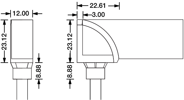
Bottom Entry Connector MJ-SF15-D5-B02SM MJ-SF15-D5-B03SFM
