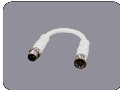
Positive Disconnected Connector Cable M12-EXT-SIG-5C-20AWG-D6-W-015
