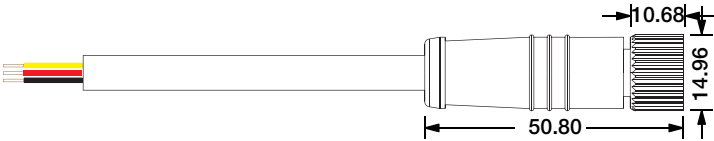
Female Connector M12-F-3C-20AWG-D6-W-0327-S
