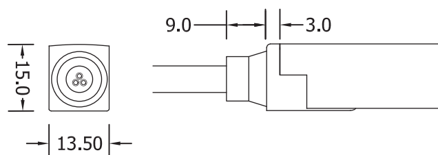
Direct Entry Connector MJ-SF10-D3-D02SM MJ-SF10-D3-D03SFM
