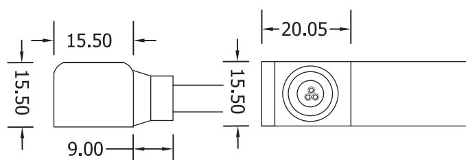
Side Entry Connector MJ-SF10-D3-S02SM MJ-SF10-D3-S03SFM
