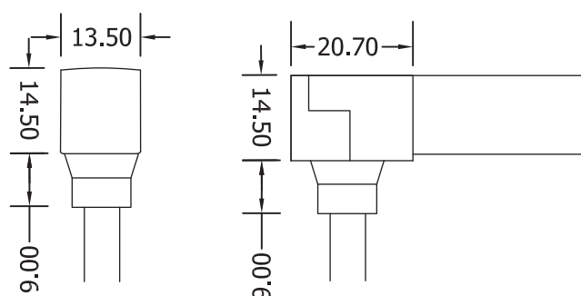
Bottom Entry Connector MJ-SF10-D3-B02SM MJ-SF10-D3-B03SFM
