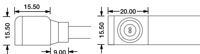
Side Entry Connector MJ-SF10-A-S01/02/03 MJ-SF10-A-S01SM MJ-SF10-A-S02SF MJ-SF10-A-S03SFM
