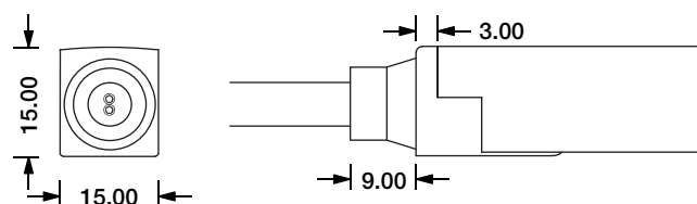
Direct Entry Connector MJ-SF10-A-D01/02/03 MJ-SF10-A-D01SM MJ-SF10-A-D02SF MJ-SF10-A-D03SFM
