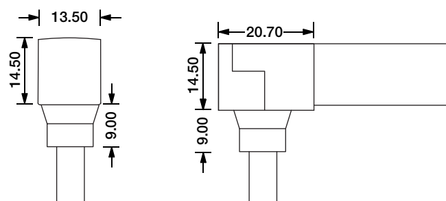
Bottom Entry Connector MJ-SF10-A-B01/02/03 MJ-SF10-A-B01SM MJ-SF10-A-B02SF MJ-SF10-A-B03SFM
