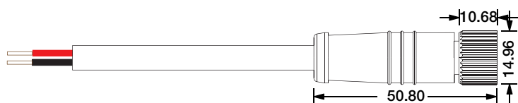
Female Connector M12-F-2C-18AWG-D6-W-0327-S
