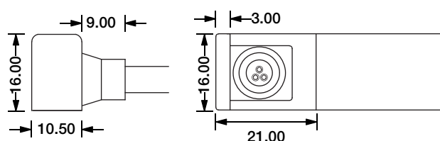
Side Entry Connector MJ-SF09-DW-S01/02/03 MJ-SF09-DW-S01SM MJ-SF09-DW-S02SF MJ-SF09-DW-S03SFM
