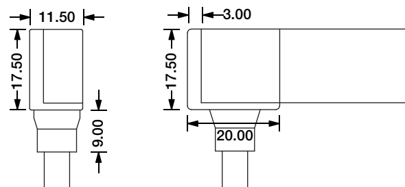
Bottom Entry Connector MJ-SF09-RGB-B01/02/03 MJ-SF09-RGB-B01SM MJ-SF09-RGB-B02SF MJ-SF09-RGB-B03SFM
