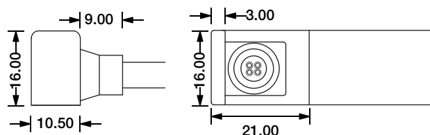
Side Entry Connector MJ-SF09-RGB-S01/02/03 MJ-SF09-RGB-S01SM MJ-SF09-RGB-S02SF MJ-SF09-RGB-S03SFM
