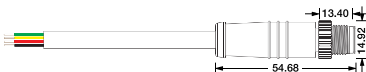
Male Connector M12-M-4C-22AWG-D5.5-W-0327-S
