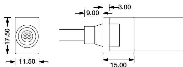
Direct Entry Connector MJ-SF09-RGB-D01/02/03 MJ-SF09-RGB-D01SM MJ-SF09-RGB-D02SF MJ-SF09-RGB-D03SFM
