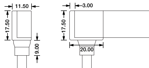
Bottom Entry Connector MJ-SF09-A-B01/02/03 MJ-SF09-A-B01SM MJ-SF09-A-B02SF MJ-SF09-A-B03SFM
