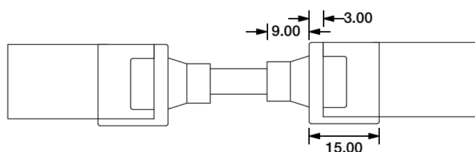
Jumper MJ-SF09-A-D-JC
