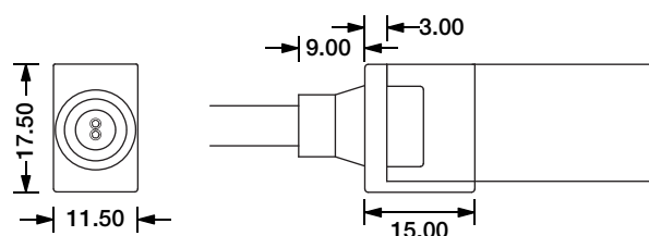
Direct Entry Connector MJ-SF09-A-D01/02/03 MJ-SF09-A-D01SM MJ-SF09-A-D02SF MJ-SF09-A-D03SFM
