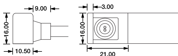
Side Entry Connector MJ-SF09-A-S01/02/03 MJ-SF09-A-S01SM MJ-SF09-A-S02SF MJ-SF09-A-S03SFM
