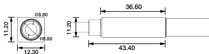
DIY Quick Connective Connector DIY-QC-FR-08-D-01/02-A
