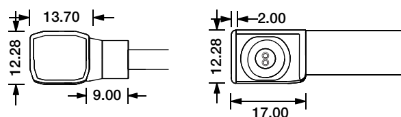
Side Entry Connector MJ-SF08-A-S01/02/03 MJ-SF08-A-S01SM MJ-SF08-A-S02SF MJ-SF09-A-S03SFM
