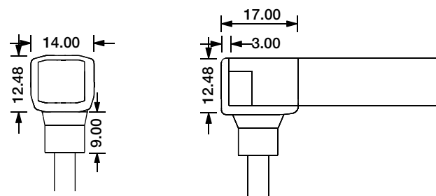
Bottom Entry Connector MJ-SF08-A-B01/02/03 MJ-SF08-A-B01SM MJ-SF08-A-B02SF MJ-SF08-A-B03SFM
