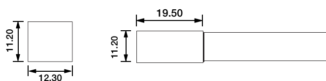
DIY Quick Connective End Cap DIY-QC-END-08
