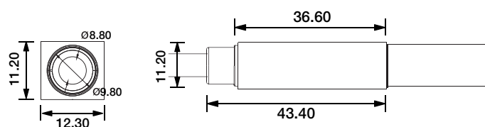
DIY Quick Connective Connector DIY-QC-FR-06-D-01/02-A
