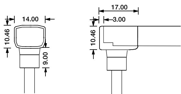
Bottom Entry Connector MJ-SF06-A-B01/02/03 MJ-SF06-A-B01SM MJ-SF06-A-B02SF MJ-SF06-A-B03SFM
