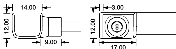
Side Entry Connector MJ-SF06-A-S01/02/03 MJ-SF06-A-S01SM MJ-SF06-A-S02SF MJ-SF06-A-S03SFM
