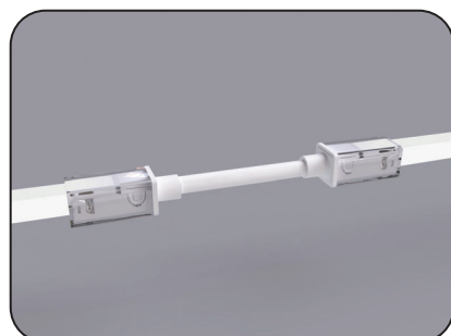
DIY Snap Extent Connector DIY-SN-EXT-06-A
