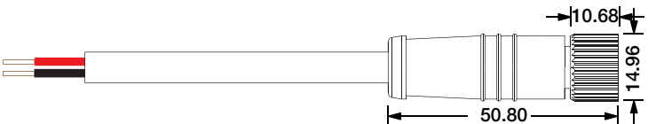
Female Connector M12-F-2C-18AWG-D6-W-0327-S
