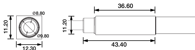
DIY Quick Connective Connector DIY-QC-FR-06-D-01/02-A
