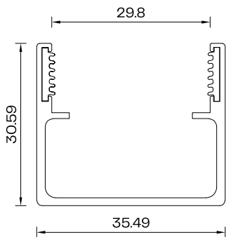
Profile Cross Section Straight Profile Scale 1:1
