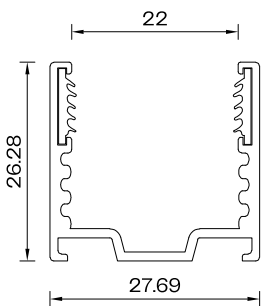
Profile Cross Section Straight Profile Scale 1:1
