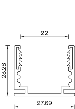
Profile Cross Section Straight Profile Scale 1:1
