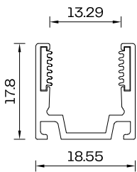
Profile Cross Section Straight Profile Scale 1:1
