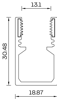
Profile Cross Section Cable Duct Profile Scale 1:1
